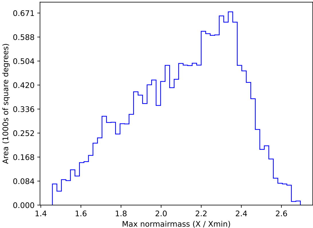
too_combined_s0.5_v3.4_10yrs WFD r band: Max normairmass
