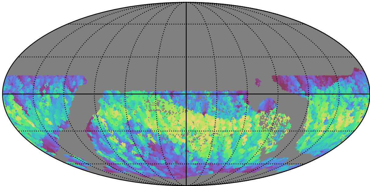
too_combined_s0.5_v3.4_10yrs WFD i band: Max normairmass
