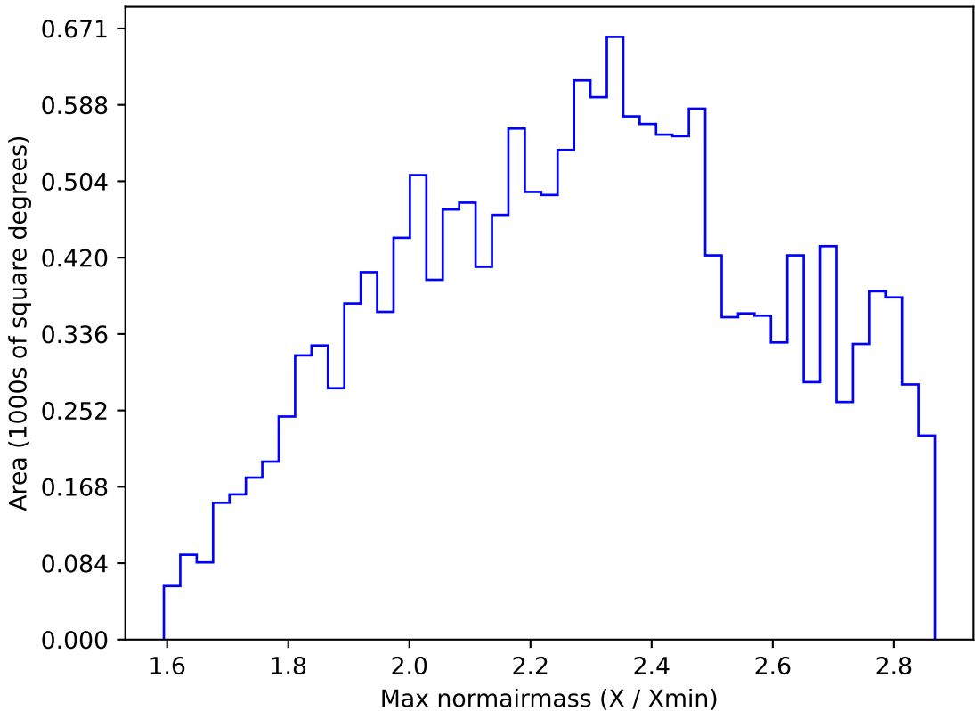
too_combined_s0.5_v3.4_10yrs WFD i band: Max normairmass
