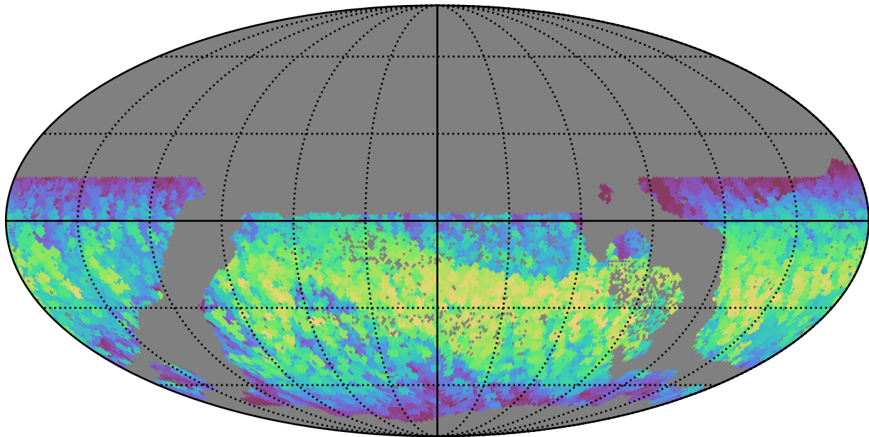
too_combined_s0.5_v3.4_10yrs WFD all bands: Max normairmass
