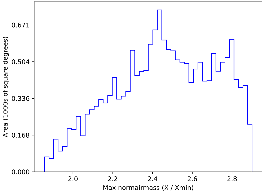
too_combined_s0.5_v3.4_10yrs WFD all bands: Max normairmass
