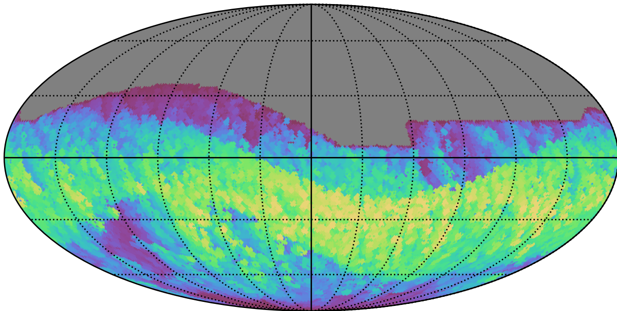
too_combined_s0.5_v3.4_10yrs All sky z band: Max normairmass
