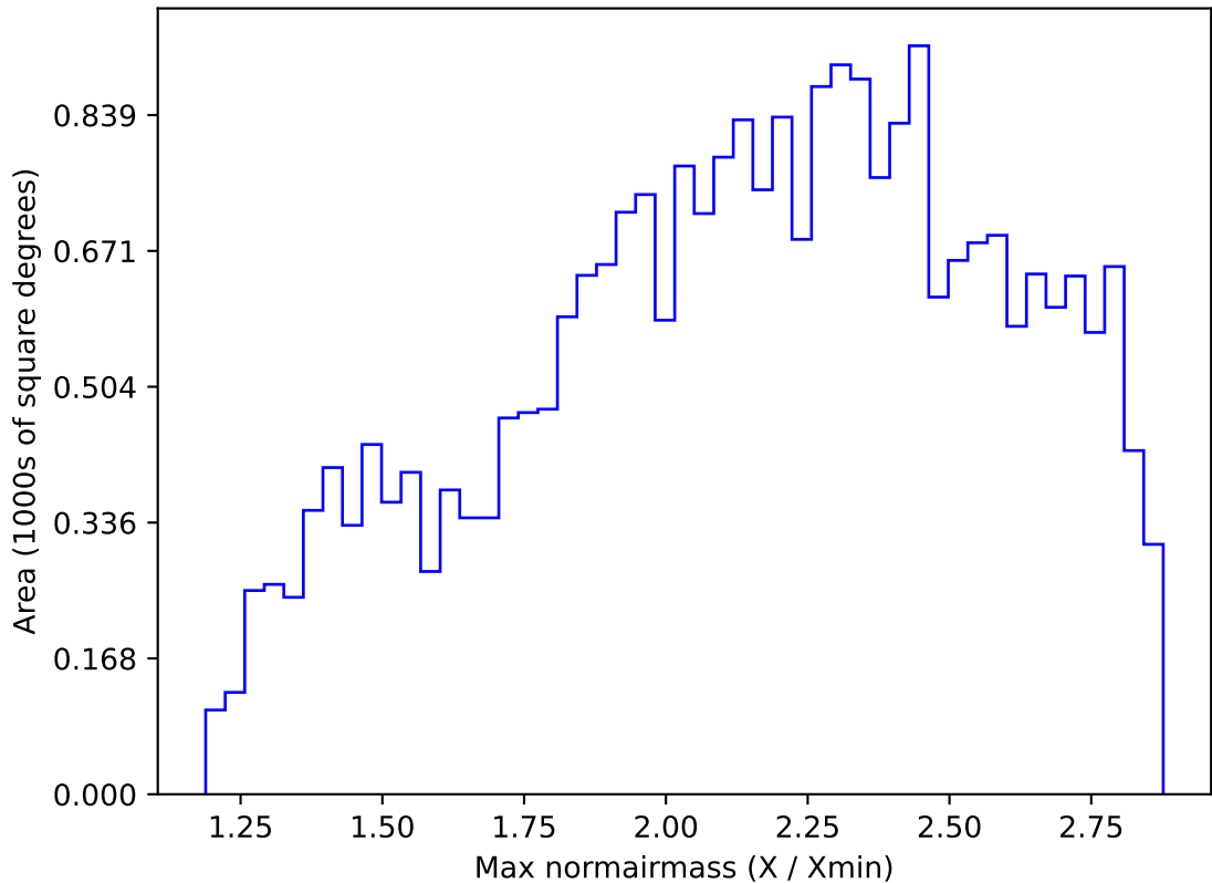
too_combined_s0.5_v3.4_10yrs All sky z band: Max normairmass
