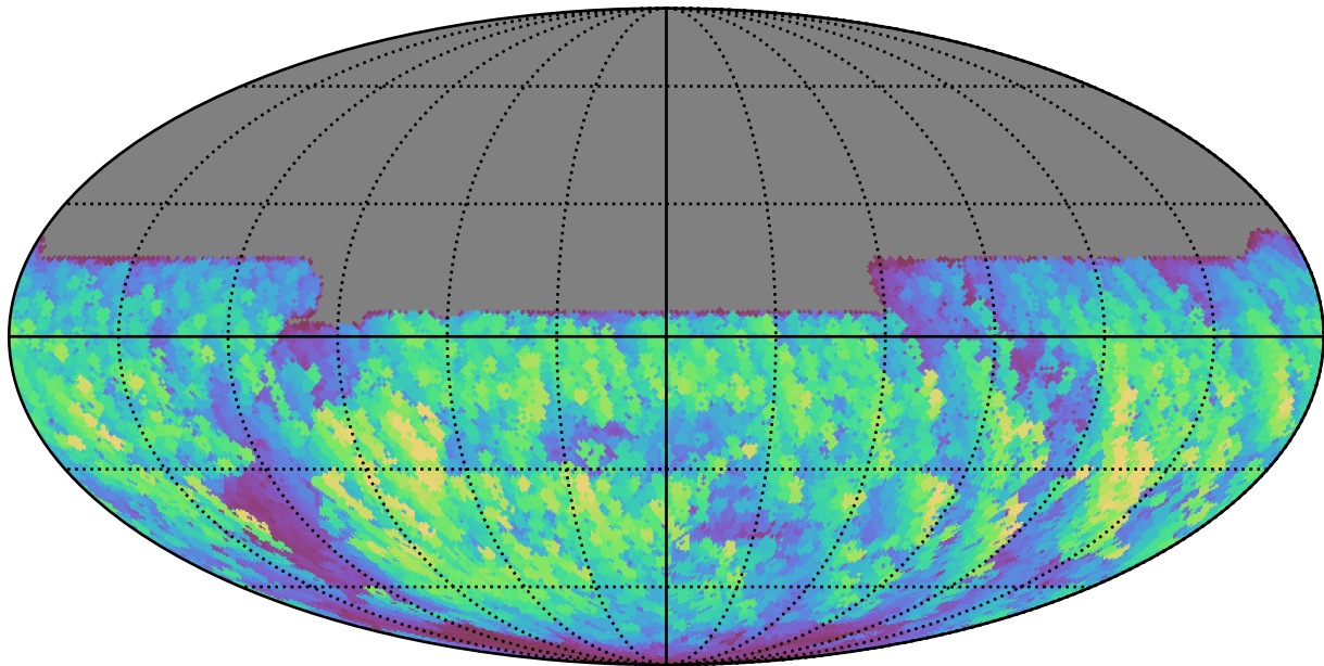
too_combined_s0.5_v3.4_10yrs All sky y band: Max normairmass
