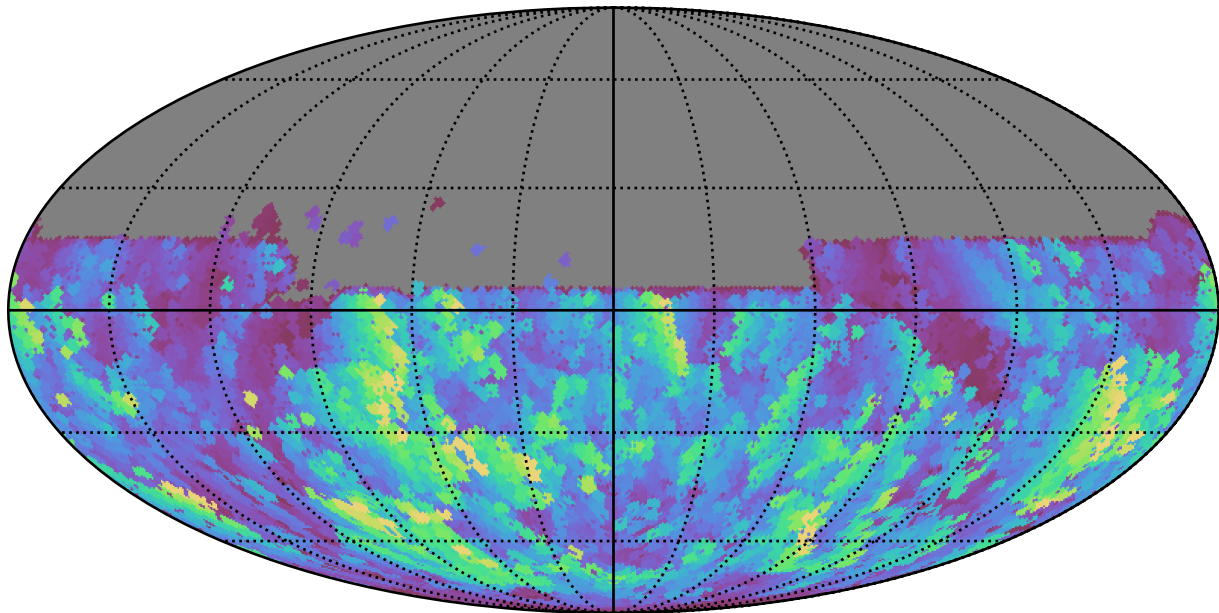
too_combined_s0.5_v3.4_10yrs All sky u band: Max normairmass
