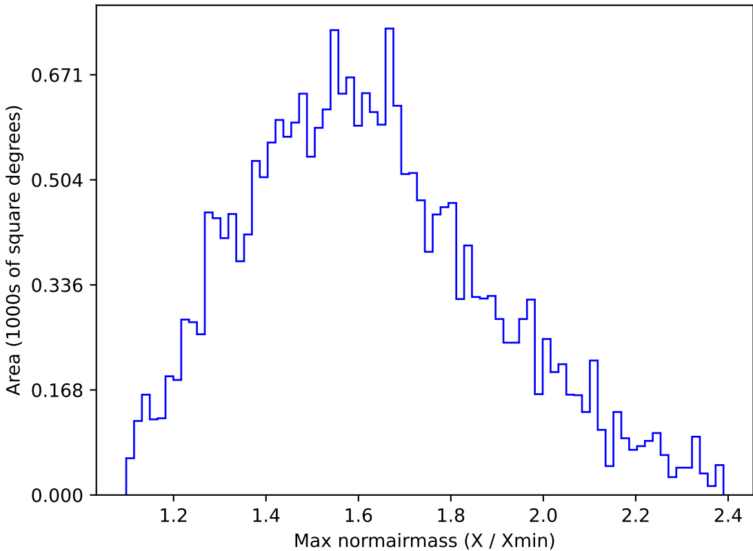
too_combined_s0.5_v3.4_10yrs All sky u band: Max normairmass
