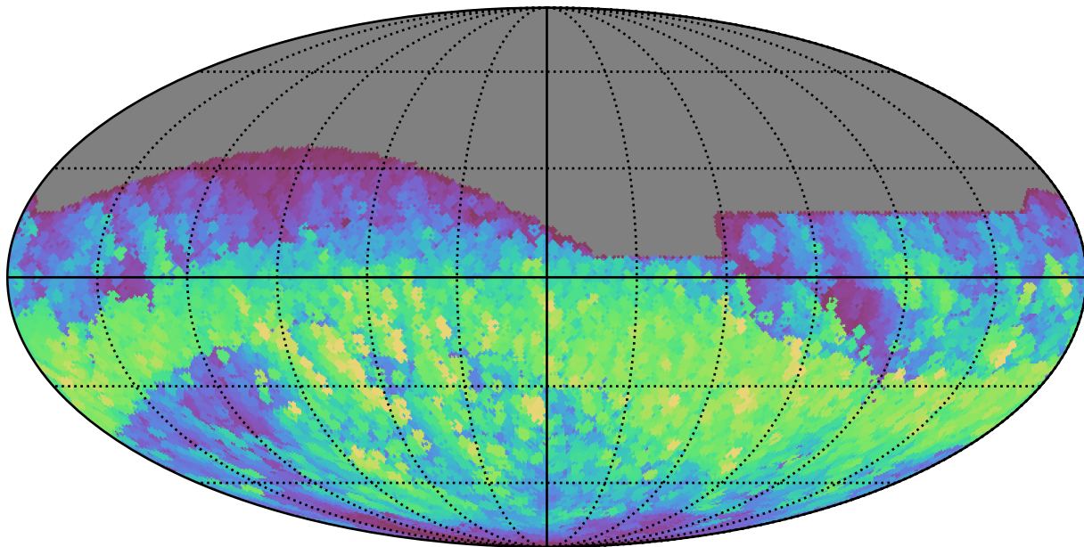
too_combined_s0.5_v3.4_10yrs All sky r band: Max normairmass
