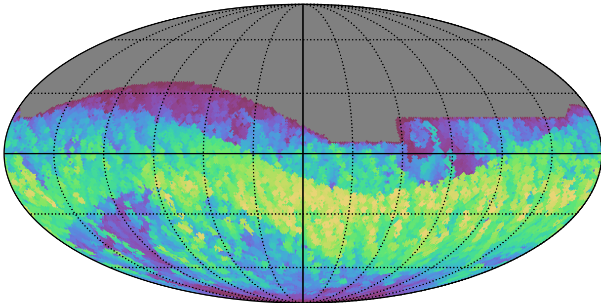
too_combined_s0.5_v3.4_10yrs All sky i band: Max normairmass
