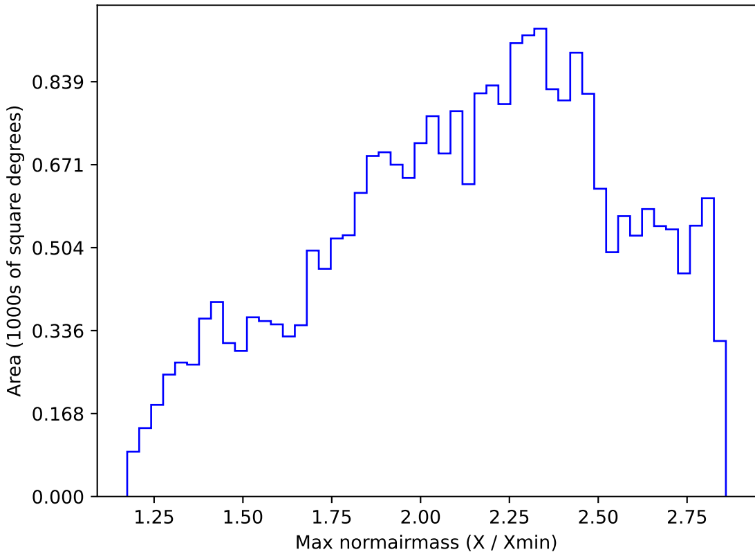
too_combined_s0.5_v3.4_10yrs All sky i band: Max normairmass
