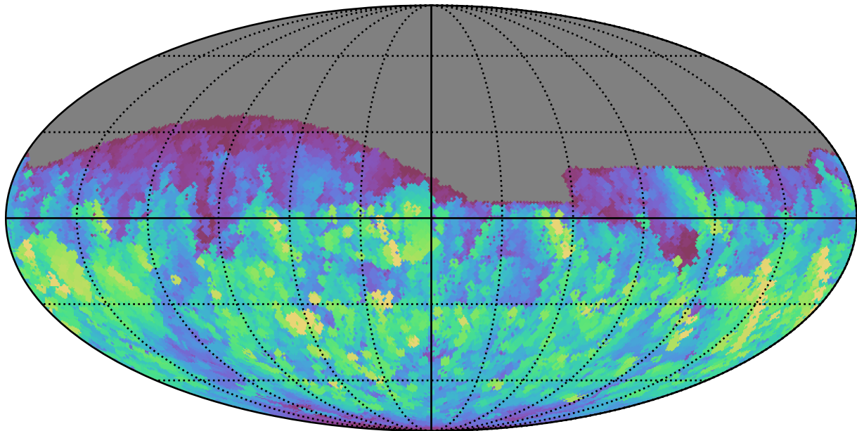
too_combined_s0.5_v3.4_10yrs All sky g band: Max normairmass
