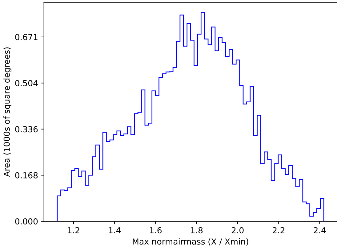
too_combined_s0.5_v3.4_10yrs All sky g band: Max normairmass
