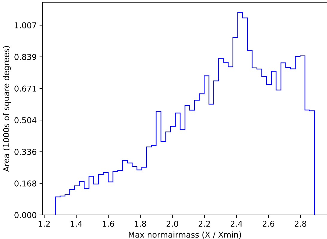
too_combined_s0.5_v3.4_10yrs All sky all bands: Max normairmass
