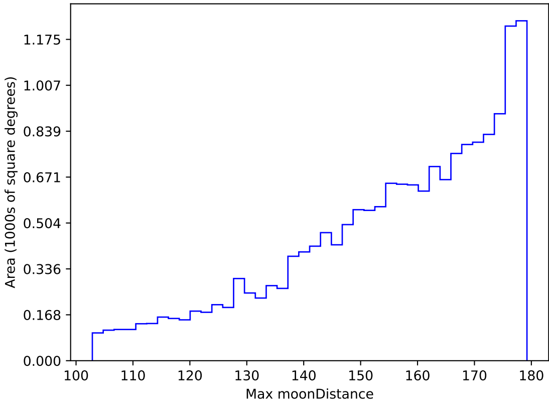
too_combined_s0.5_v3.4_10yrs WFD i band: Max moonDistance
