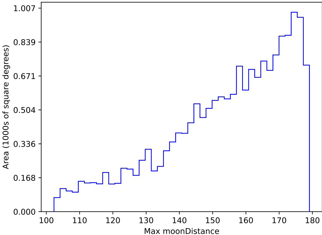
too_combined_s0.5_v3.4_10yrs WFD g band: Max moonDistance
