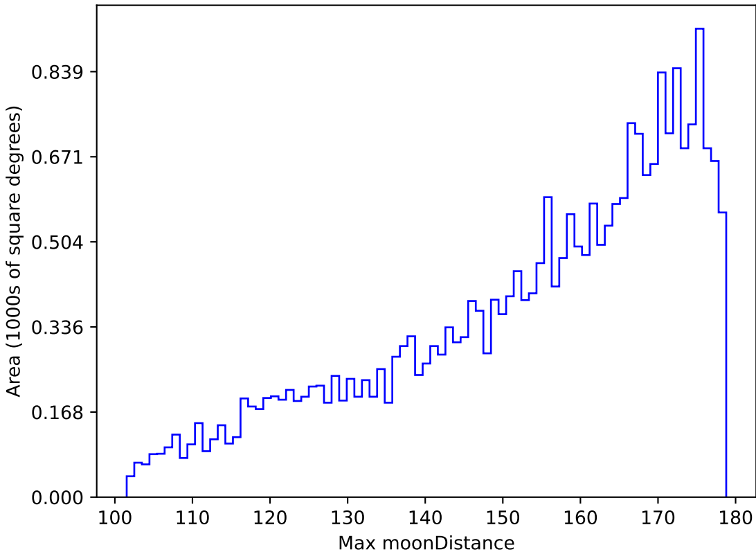
too_combined_s0.5_v3.4_10yrs All sky z band: Max moonDistance
