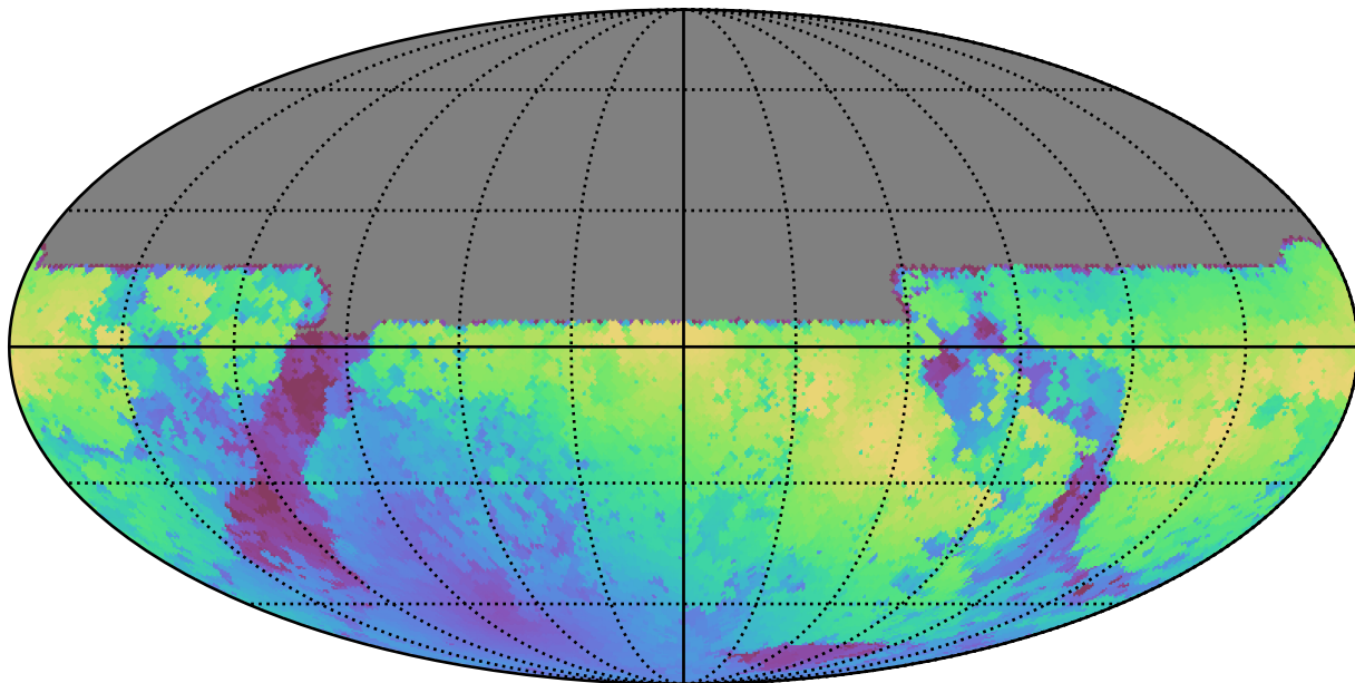
too_combined_s0.5_v3.4_10yrs All sky y band: Max moonDistance
