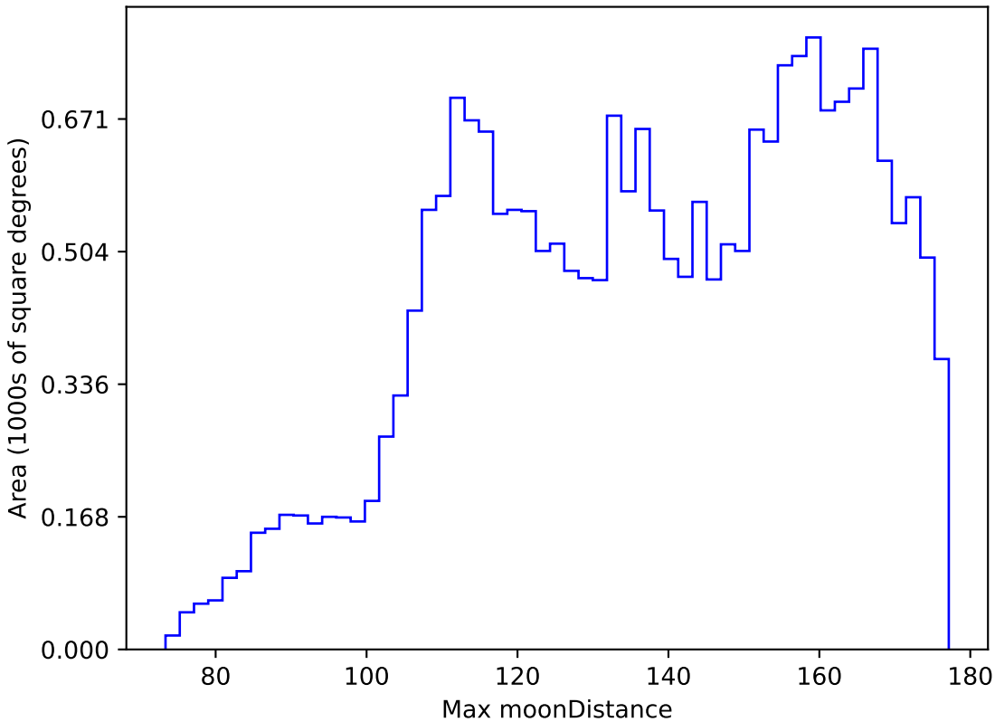
too_combined_s0.5_v3.4_10yrs All sky y band: Max moonDistance
