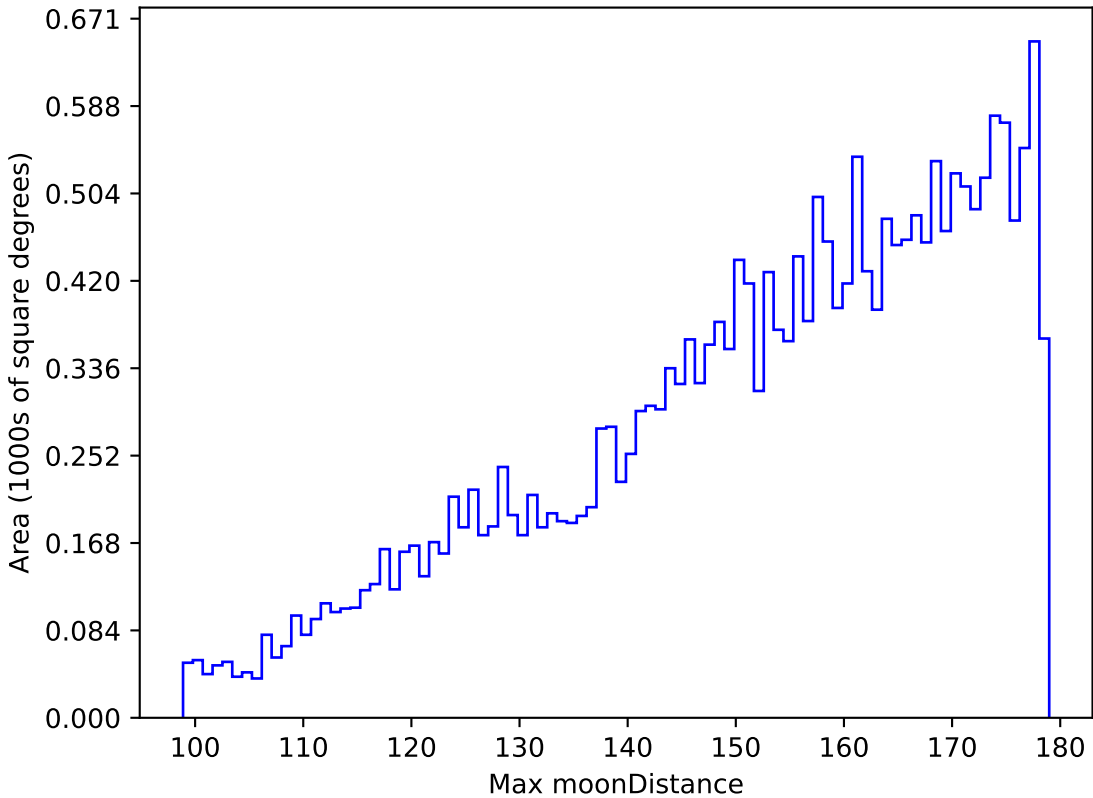
too_combined_s0.5_v3.4_10yrs All sky u band: Max moonDistance
