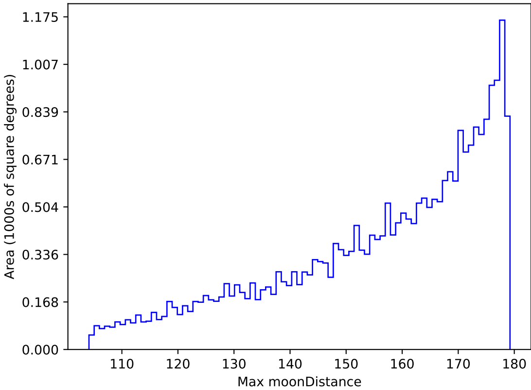
too_combined_s0.5_v3.4_10yrs All sky r band: Max moonDistance
