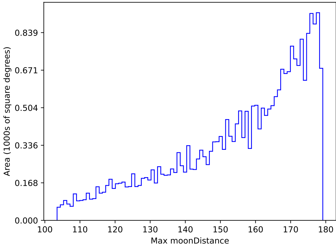
too_combined_s0.5_v3.4_10yrs All sky i band: Max moonDistance
