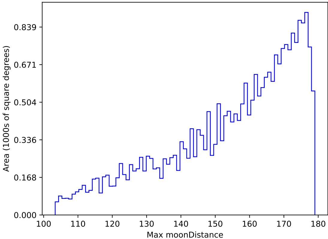
too_combined_s0.5_v3.4_10yrs All sky g band: Max moonDistance
