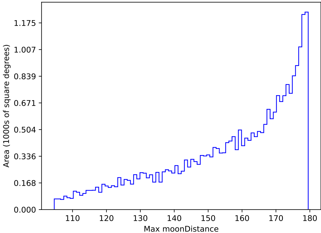
too_combined_s0.5_v3.4_10yrs All sky all bands: Max moonDistance
