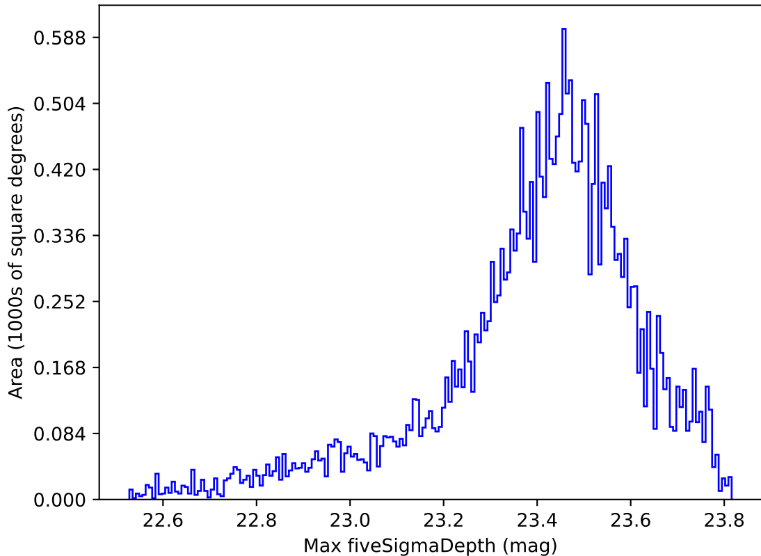
too_combined_s0.5_v3.4_10yrs Yr 1 z band: Max fiveSigmaDepth
