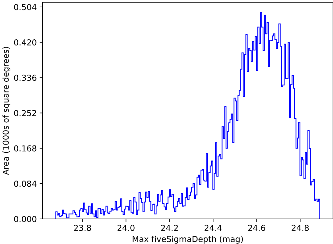
too_combined_s0.5_v3.4_10yrs Yr 1 r band: Max fiveSigmaDepth
