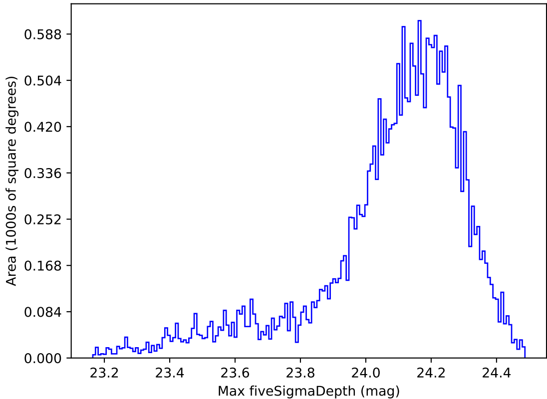
too_combined_s0.5_v3.4_10yrs Yr 1 i band: Max fiveSigmaDepth
