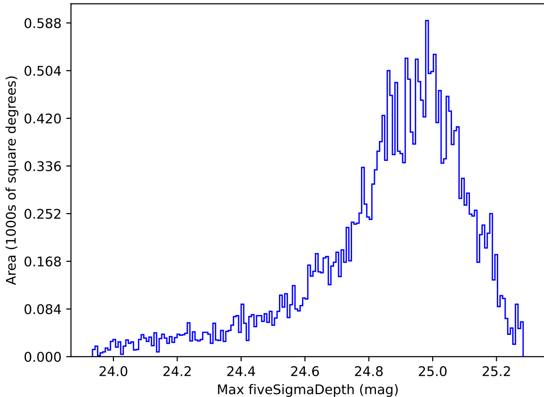
too_combined_s0.5_v3.4_10yrs Yr 1 g band: Max fiveSigmaDepth
