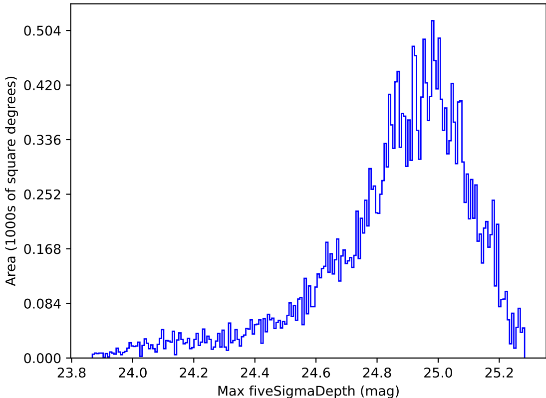
too_combined_s0.5_v3.4_10yrs Yr 1 all bands: Max fiveSigmaDepth
