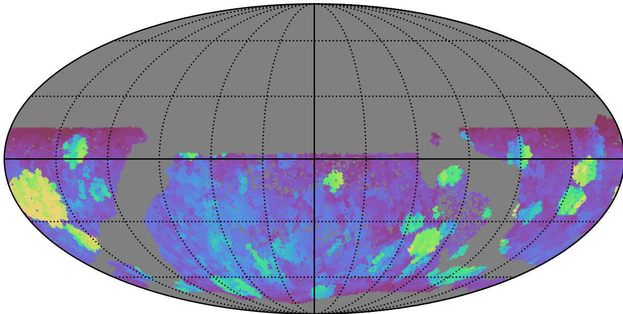
too_combined_s0.5_v3.4_10yrs WFD r band: Max fiveSigmaDepth
