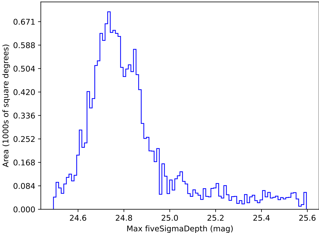
too_combined_s0.5_v3.4_10yrs WFD r band: Max fiveSigmaDepth
