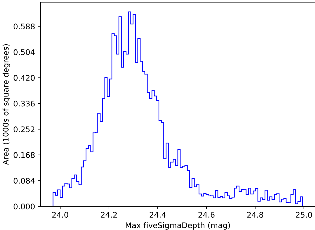
too_combined_s0.5_v3.4_10yrs WFD i band: Max fiveSigmaDepth
