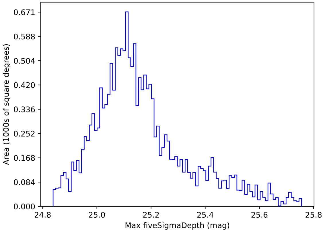
too_combined_s0.5_v3.4_10yrs WFD all bands: Max fiveSigmaDepth
