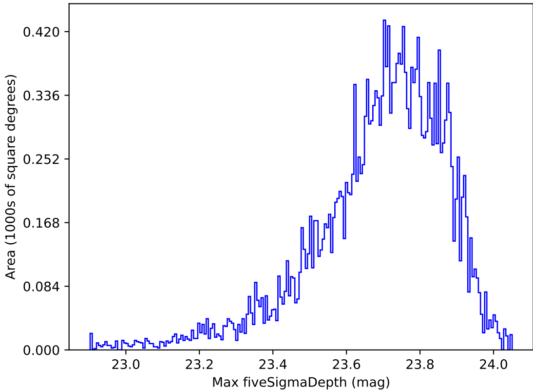
too_combined_s0.5_v3.4_10yrs All sky u band: Max fiveSigmaDepth
