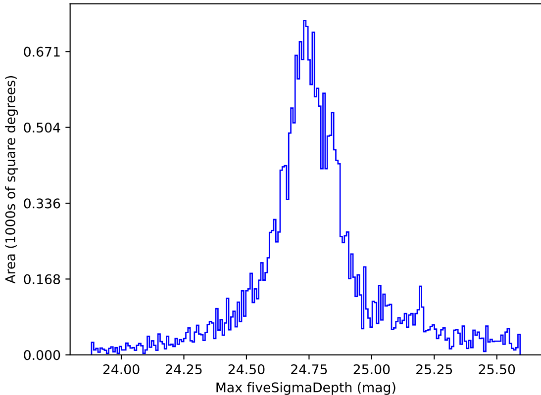
too_combined_s0.5_v3.4_10yrs All sky r band: Max fiveSigmaDepth
