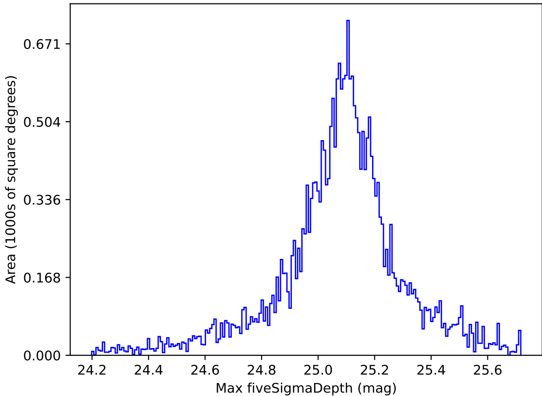
too_combined_s0.5_v3.4_10yrs All sky g band: Max fiveSigmaDepth
