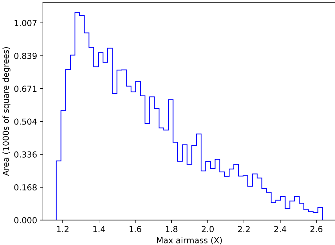
too_combined_s0.5_v3.4_10yrs Yr 1 y band: Max airmass
