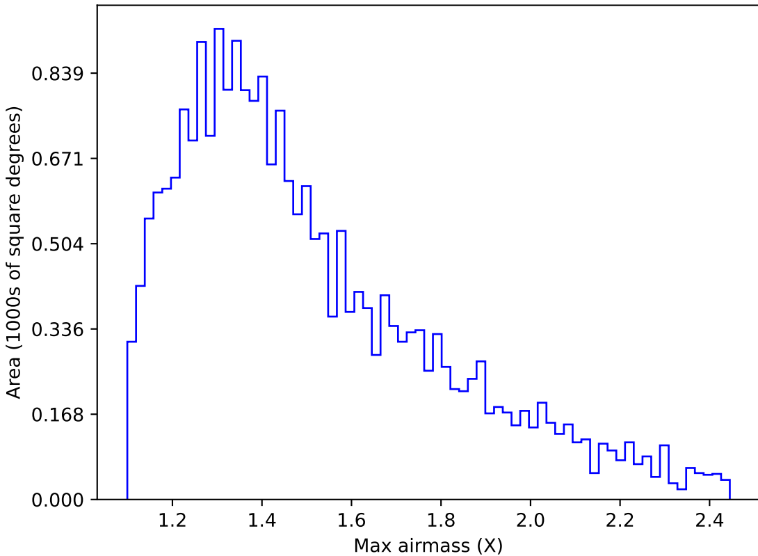
too_combined_s0.5_v3.4_10yrs Yr 1 u band: Max airmass
