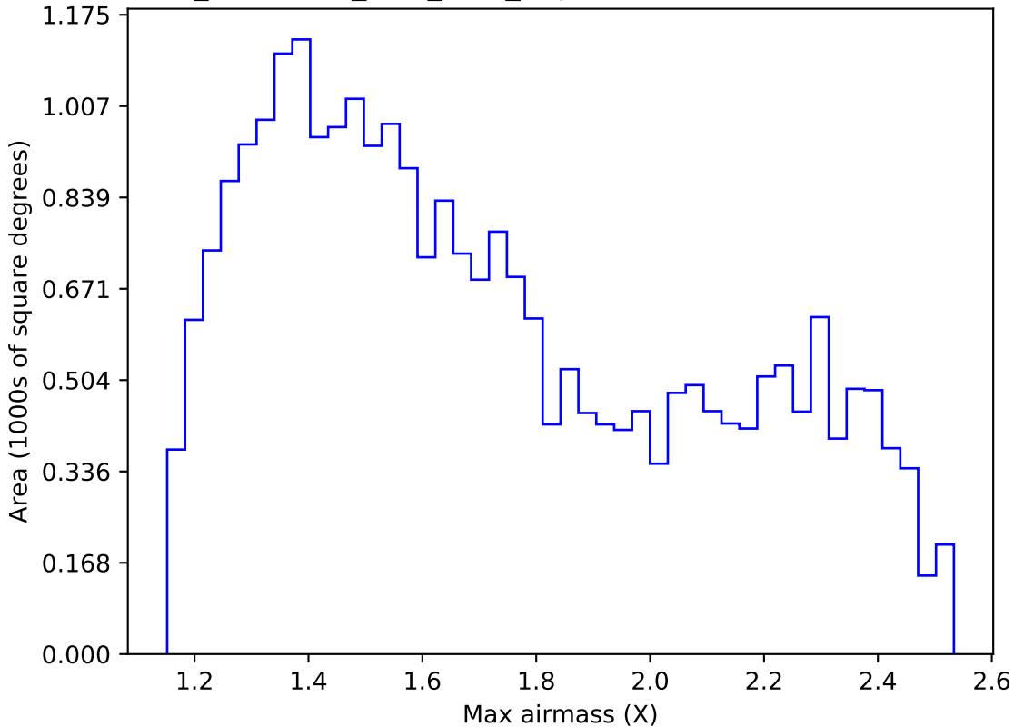
too_combined_s0.5_v3.4_10yrs Yr 1 r band: Max airmass
