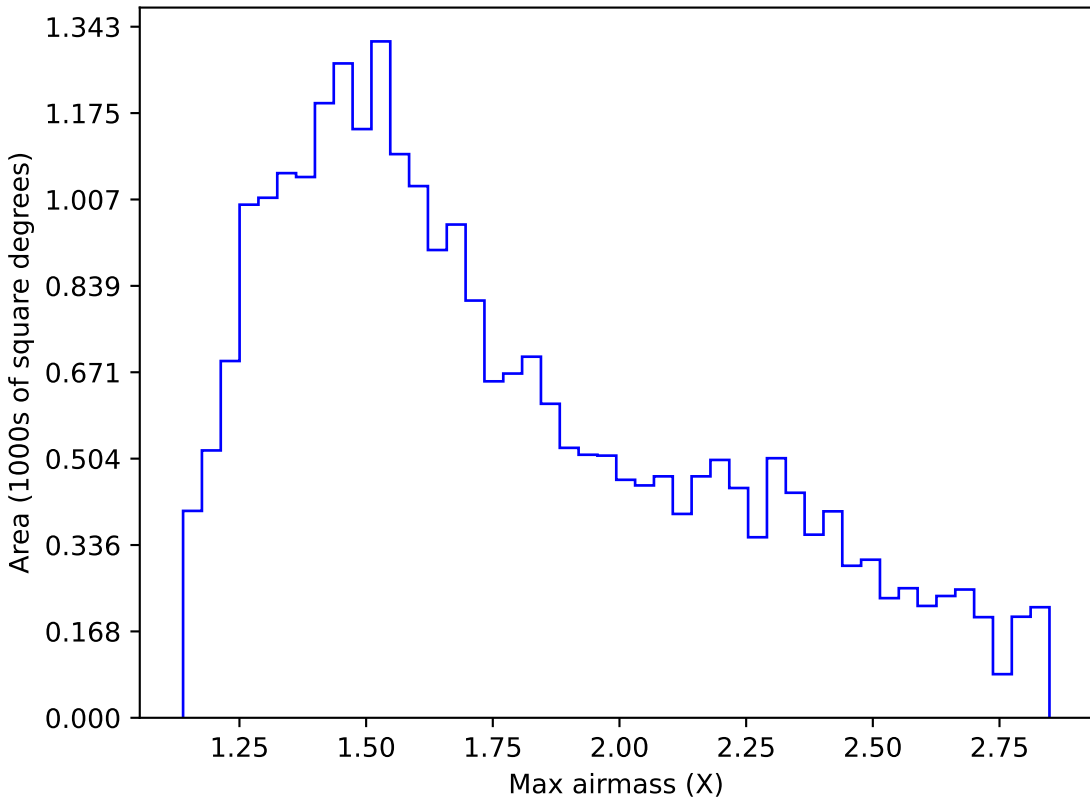
too_combined_s0.5_v3.4_10yrs Yr 1 i band: Max airmass
