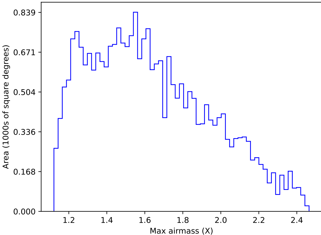
too_combined_s0.5_v3.4_10yrs Yr 1 g band: Max airmass
