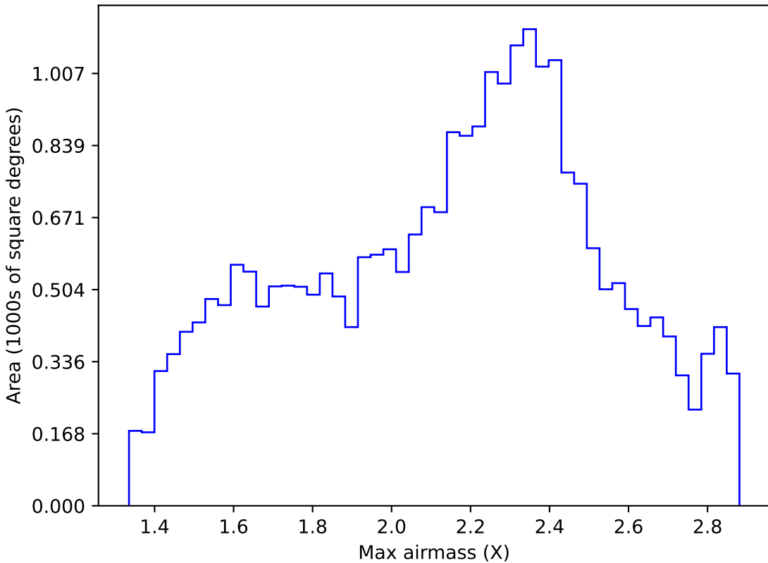
too_combined_s0.5_v3.4_10yrs Yr 1 all bands: Max airmass
