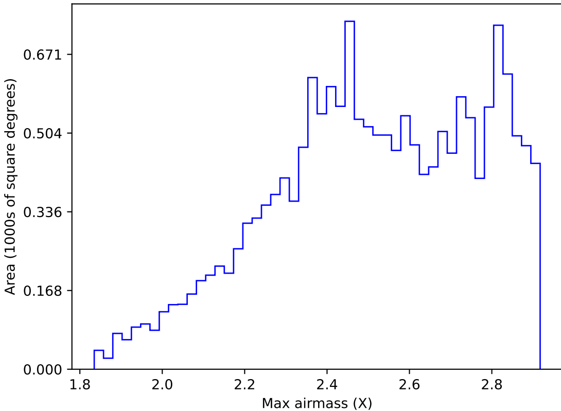
too_combined_s0.5_v3.4_10yrs WFD z band: Max airmass
