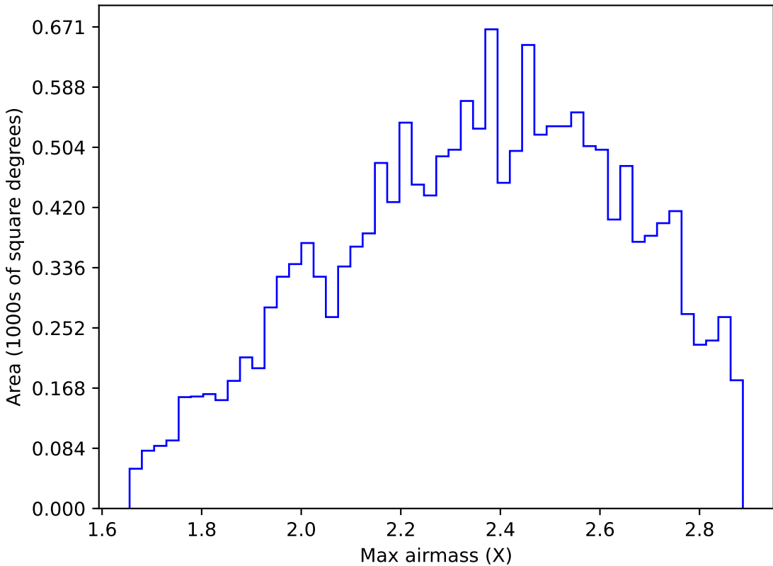
too_combined_s0.5_v3.4_10yrs WFD y band: Max airmass
