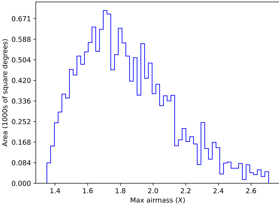
too_combined_s0.5_v3.4_10yrs WFD u band: Max airmass
