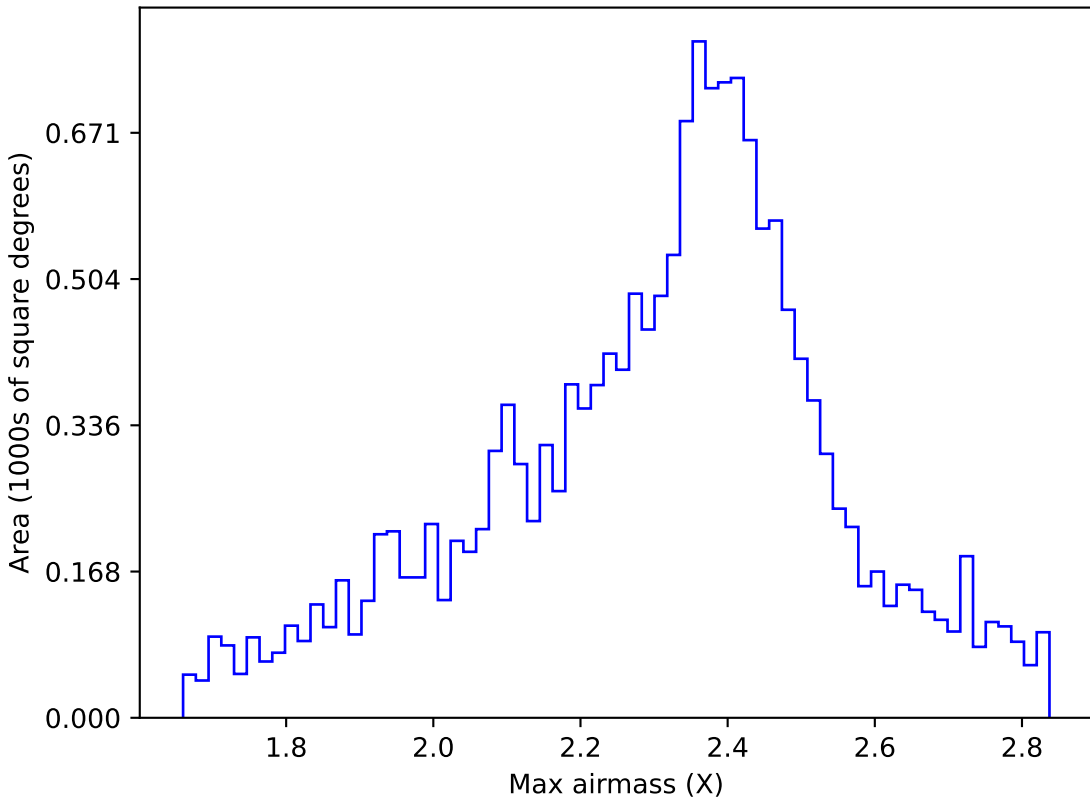
too_combined_s0.5_v3.4_10yrs WFD r band: Max airmass
