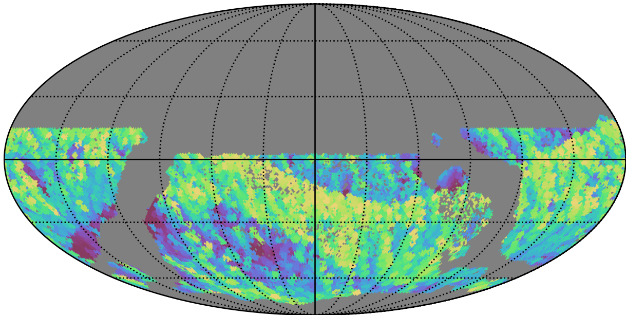
too_combined_s0.5_v3.4_10yrs WFD i band: Max airmass
