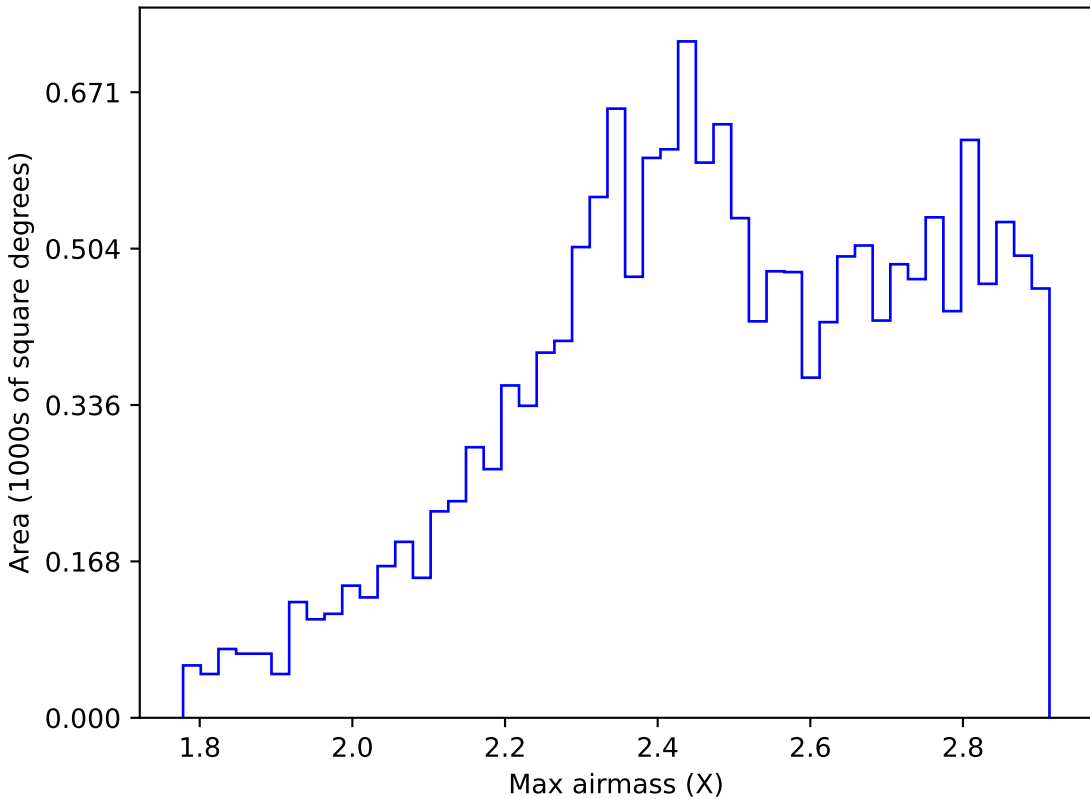
too_combined_s0.5_v3.4_10yrs WFD i band: Max airmass
